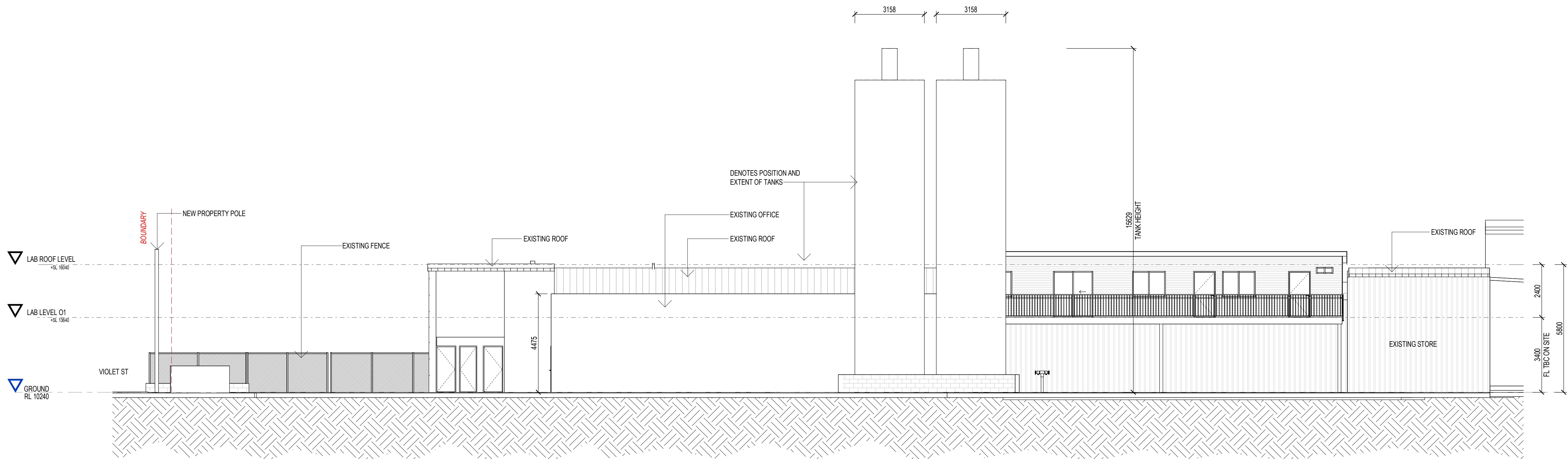
2 - ELEV SOUTH 1 : 100
